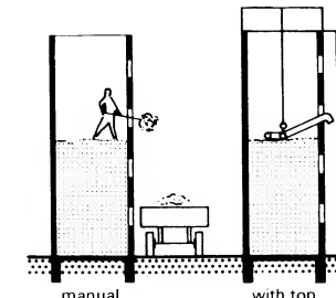
14 Tower silo: extraction
